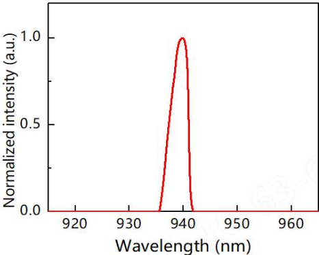
⚙ Spectral characteristics
