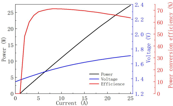
⚙ Power-Current-Voltage-Efficiency
