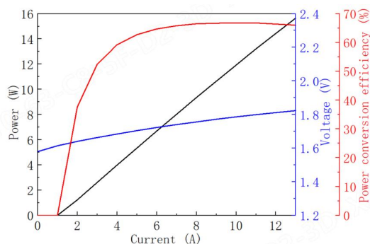
⚙ Power-Current-Voltage-Efficiency
