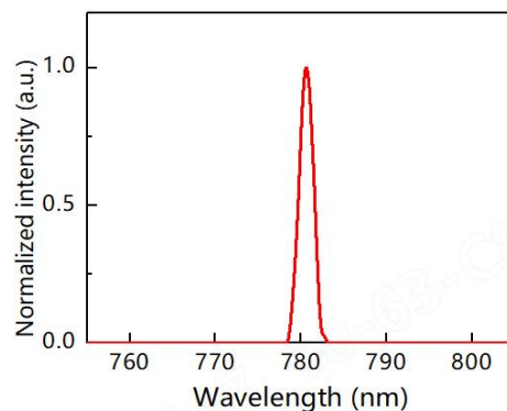
⚙ Spectral characteristics
