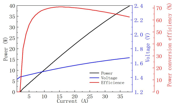
Power-Current-Voltage-Efficiency
