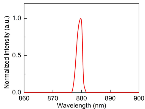
⚙ Spectral characteristics
