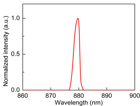
⚙ Spectral characteristics
