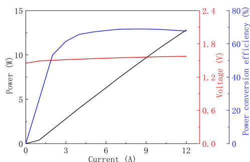
⚙ Power-Current-Voltage-Efficiency
