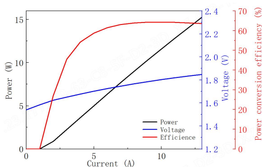
⚙ Power-Current-Voltage-Efficiency
