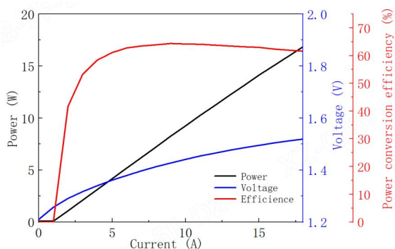
⚙ Power-Current-Voltage-Efficiency
