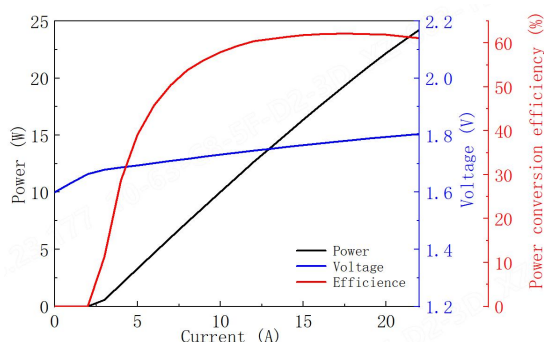
⚙ Power-Current-Voltage-Efficiency
