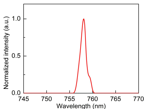
⚙ Spectral characteristics
