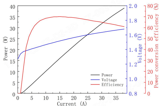
☉ Power-Current-Voltage-Efficiency
