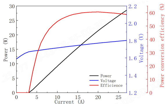
⚙ Power-Current-Voltage-Efficiency
