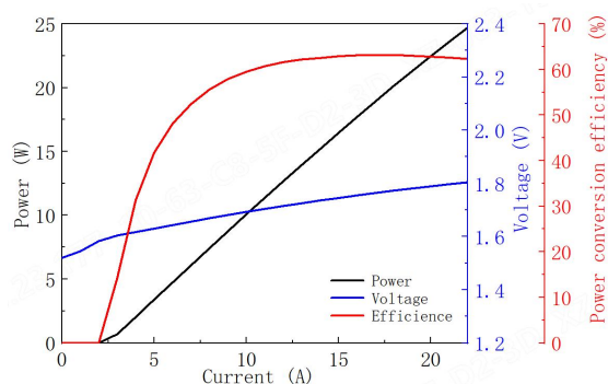
⚙ Power-Current-Voltage-Efficiency
