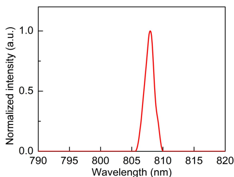
⚙ Spectral characteristics
