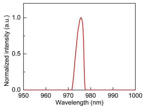
Spectral characteristics
