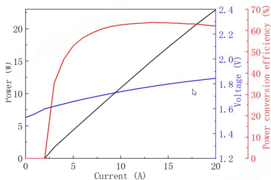
⚙ Power-Current-Voltage-Efficiency
