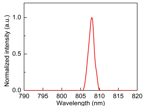
⚙ Spectral characteristics
