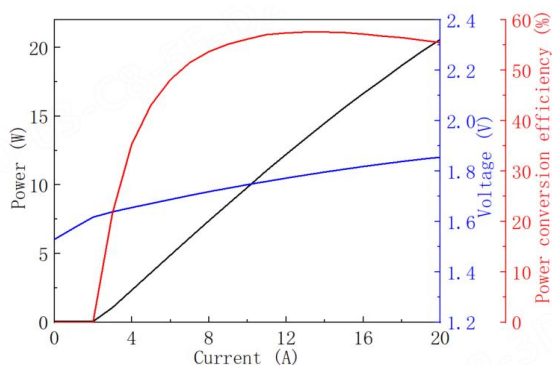
⚙ Power-Current-Voltage-Efficiency
