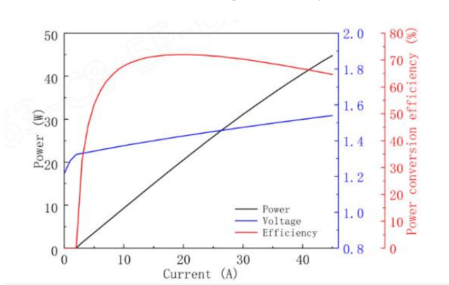
⚙ Power-Current-Voltage-Efficiency
