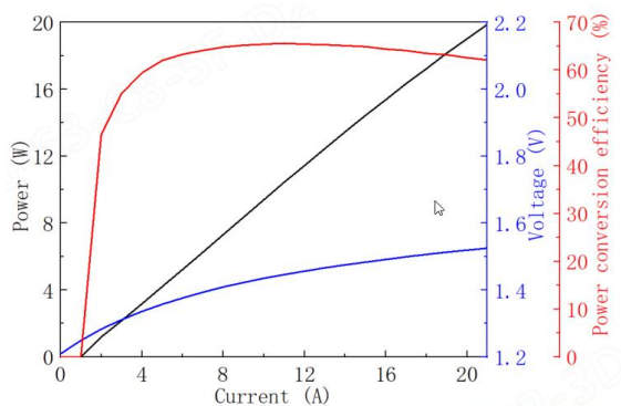
Power-Current-Voltage-Efficiency
