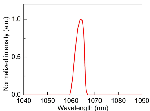
Spectral characteristics
