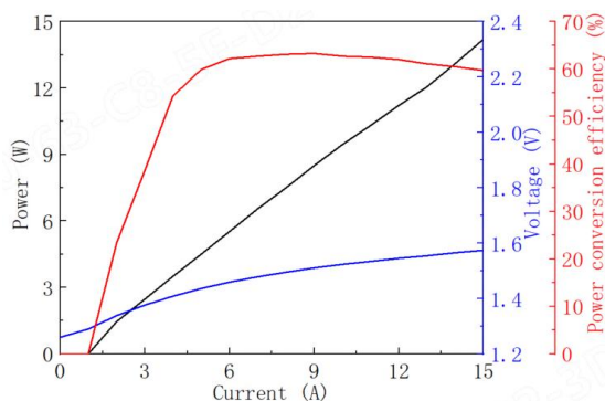
⚙ Power-Current-Voltage-Efficiency
