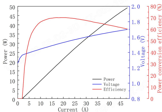
Power-Current-Voltage-Efficiency
