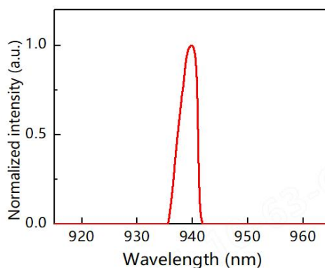
Spectral characteristics
