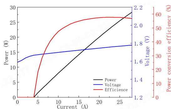
⚙ Power-Current-Voltage-Efficiency
