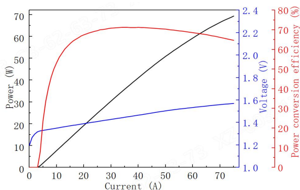
Power-Current-Voltage-Efficiency
