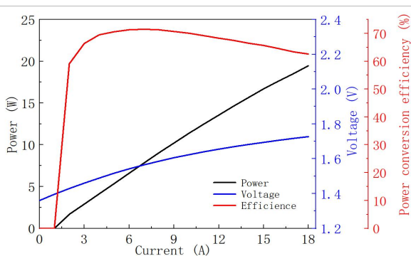
☼ Power-Current-Voltage-Efficiency
