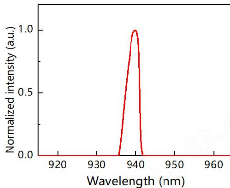
☼ Spectral characteristics
