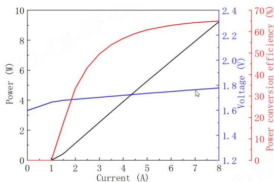
⚙ Power-Current-Voltage-Efficiency
