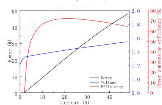
Power-Current-Voltage-Efficiency
