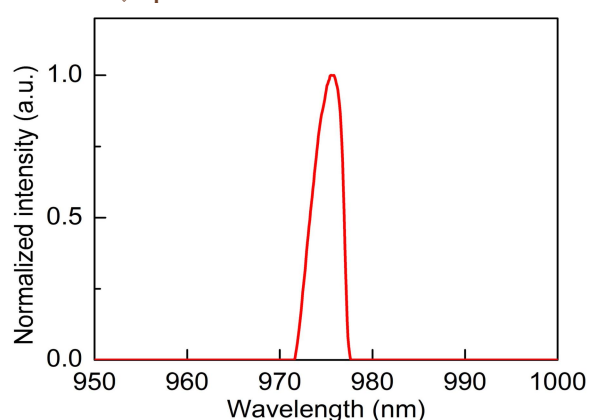
Spectral characteristics
