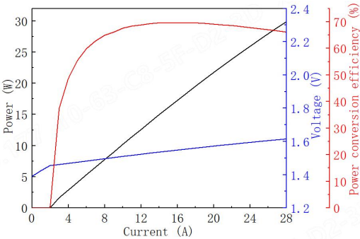
Power-Current-Voltage-Efficiency
