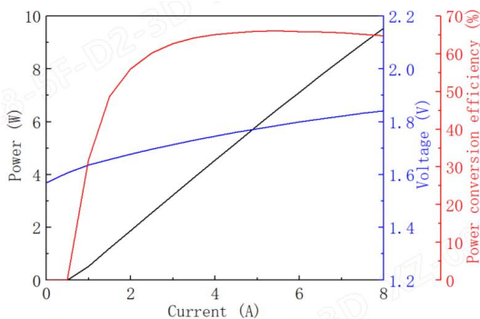
Power-Current-Voltage-Efficiency
