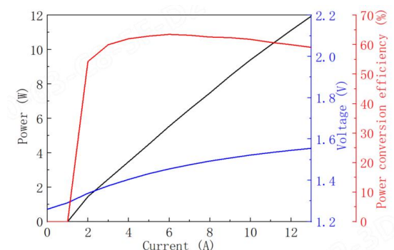
⚙ Power-Current-Voltage-Efficiency
