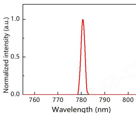
⚙ Spectral characteristics
