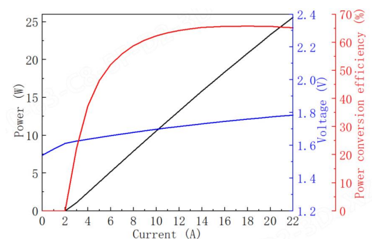
⚙ Power-Current-Voltage-Efficiency
